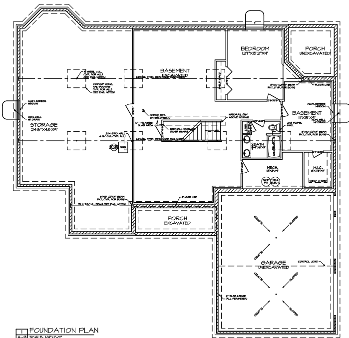
1 FOUNDATION PLAN A-3 SCALE: 1/4"=1'-0"
